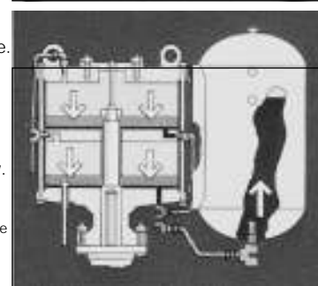
CORRECT FLUID LEVEL FOR LG TYPE PISTON
